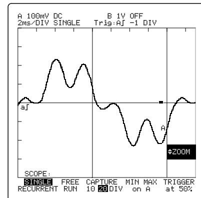
Figure 2A. Distorted current waveform
